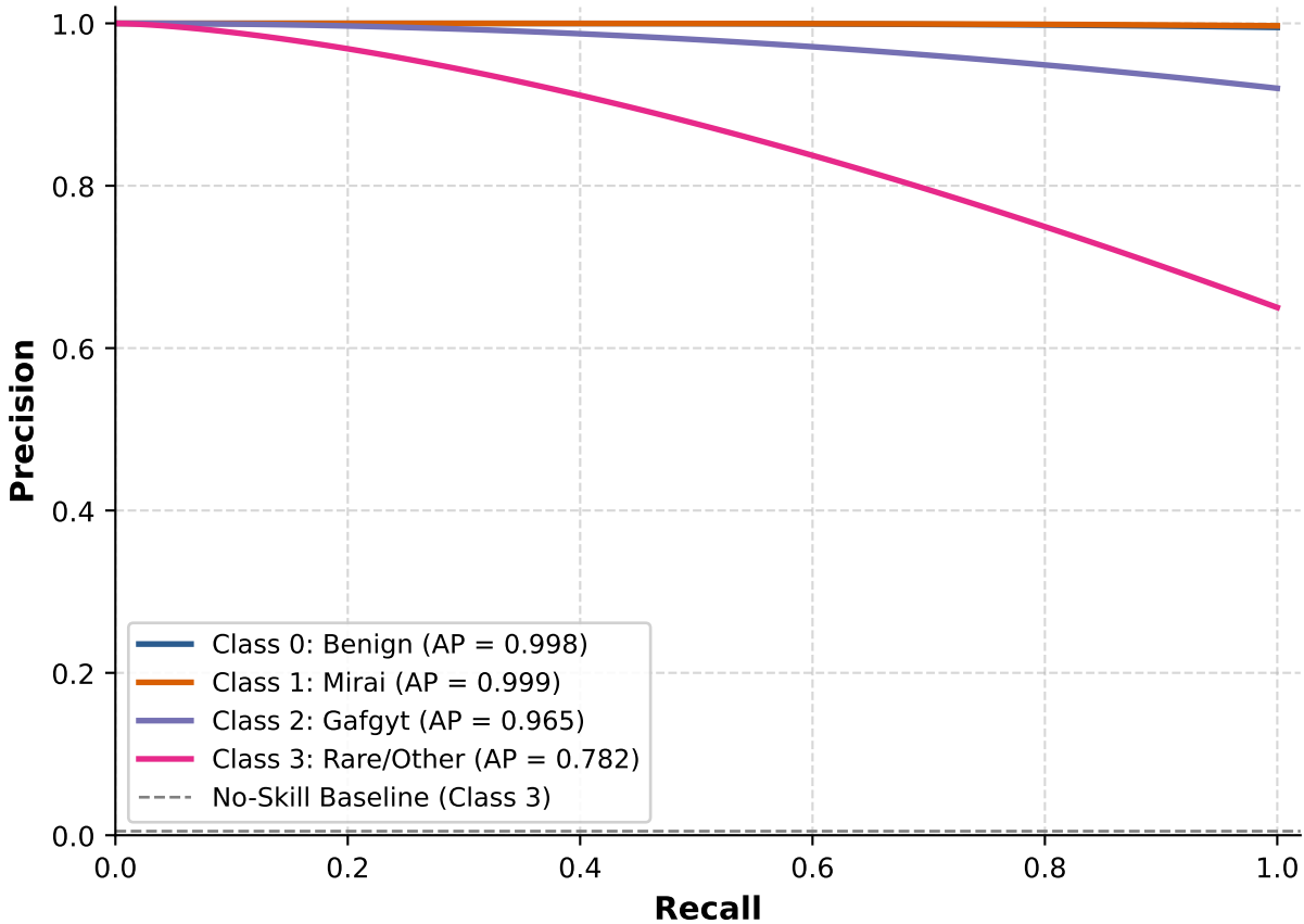
Multi-Class Precision-Recall Curves (Proposed HolisticELF)
